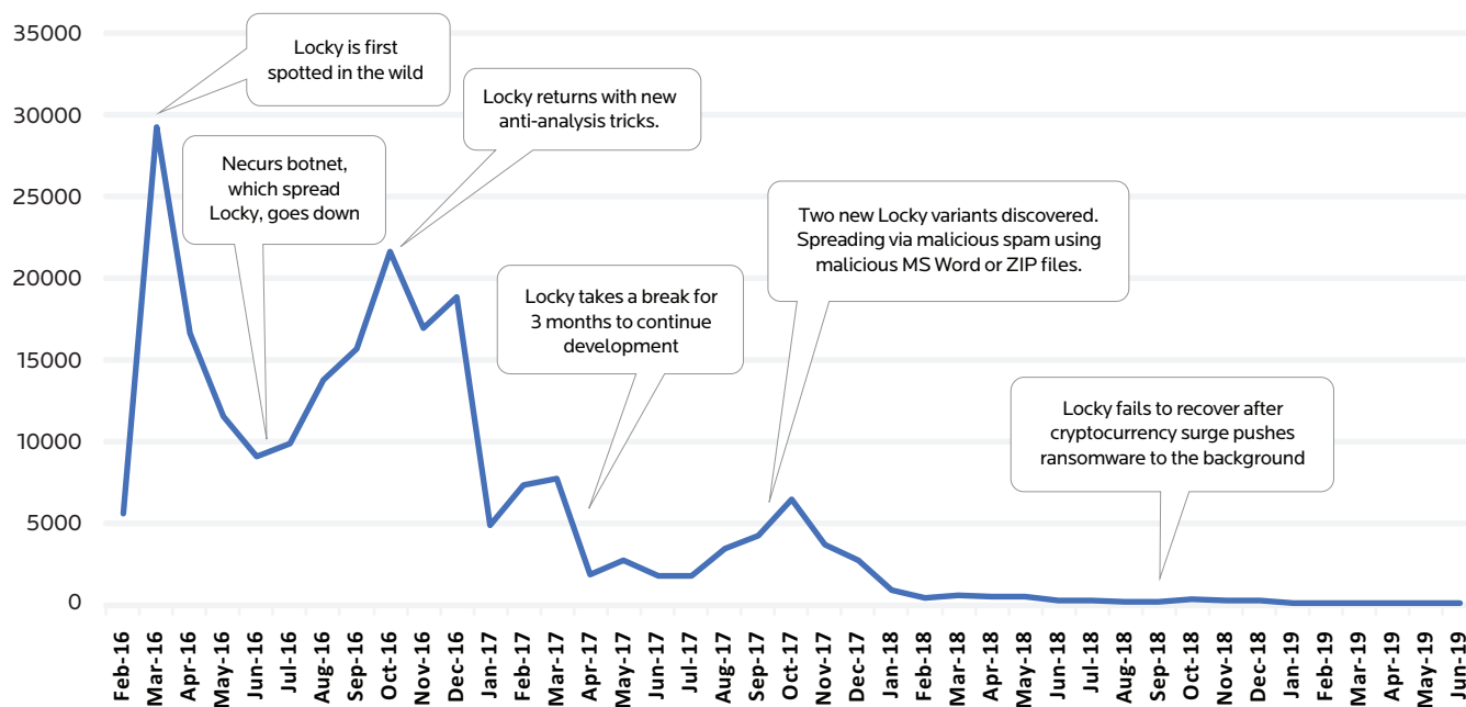
Figure 14. Locky detections
