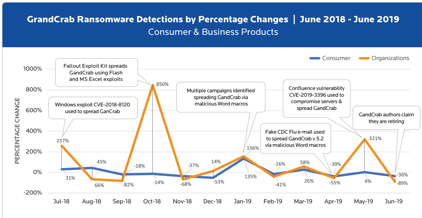
Figure 7. GandCrab evolution
